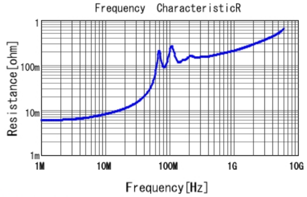
■ GRM3195C2A333JA01 R DCOV, 25degC
