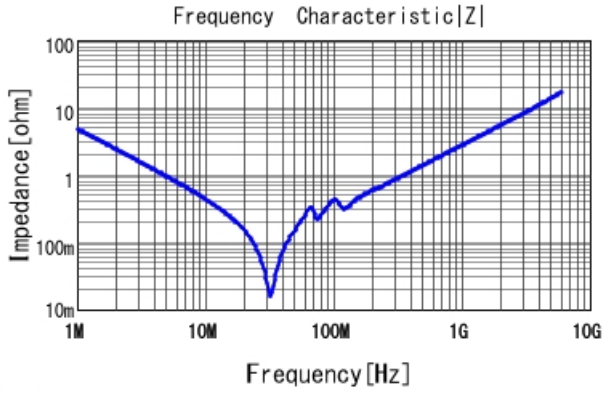
■ GRM3195C2A333JA01 |Z| DCOV, 25degC
