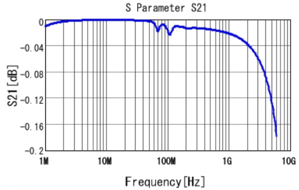
■ GRM3195C2A333JA01 S21 DCOV, 25degC
