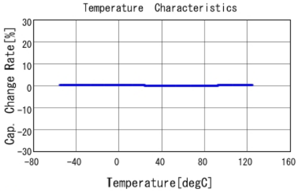
■ GRM3195C2A333JA01 C-Temp. capchange, DCOV, AC1Vrms
