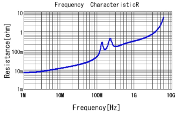
■ GRM3195C2A822JA01 R DCOV, 25degC
