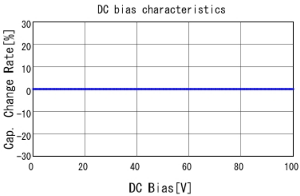
■ GRM3195C2A822JA01 C-DC bias capchange, 25.0degC, AC1V
