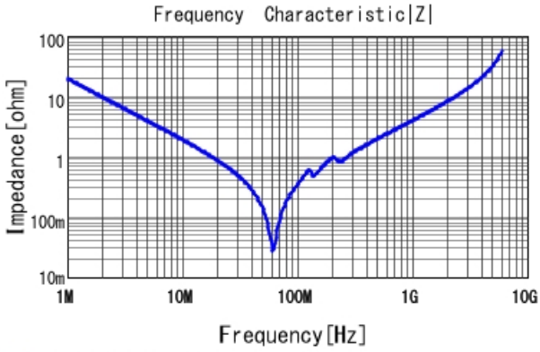
■ GRM3195C2A822JA01 |Z| DCOV, 25degC
