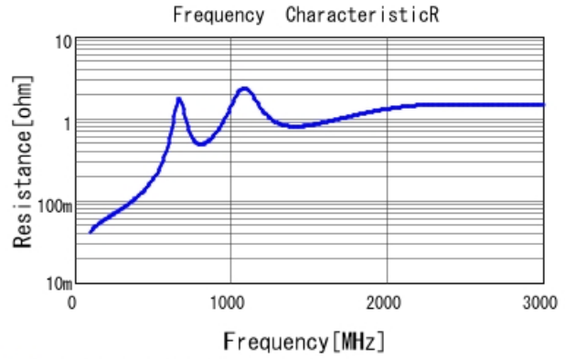
■ GRM31A5C3A391JWA1 R DCOV, 25degC
