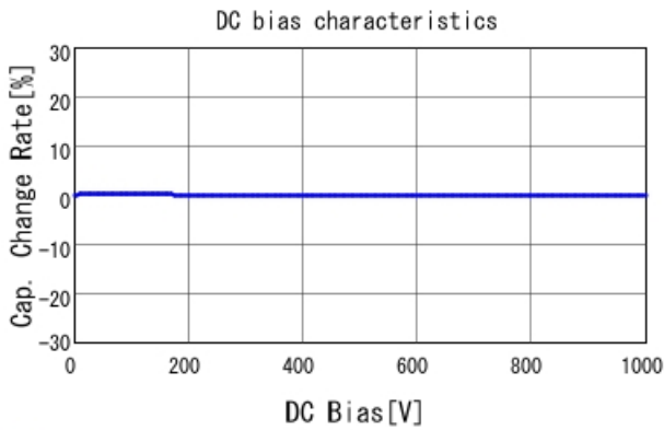
■ GRM31A5C3A391JWA1 C-DC bias capchange, 25.0degC, AC1V
