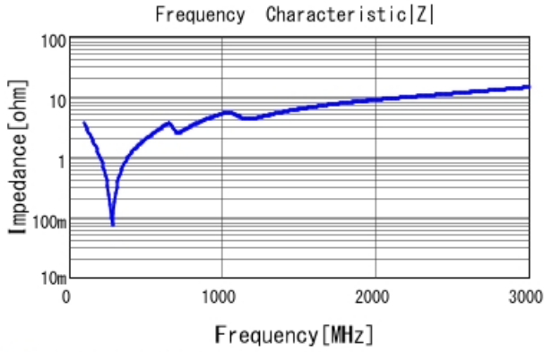
■ GRM31A5C3A391JWA1 |Z| DCOV, 25degC
