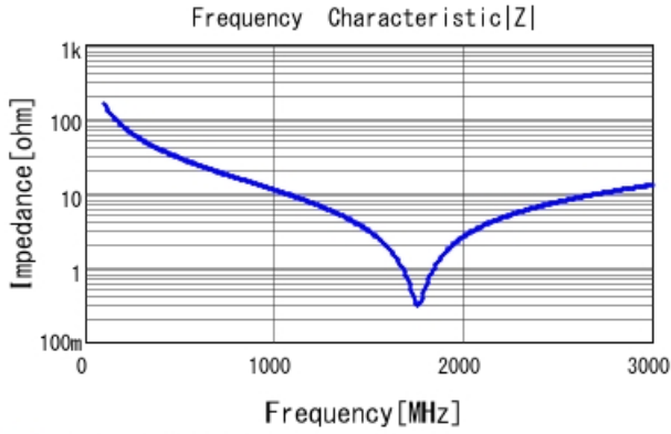
■ GRM31A7U2J100JW31 |Z| DC0V, 25degC
