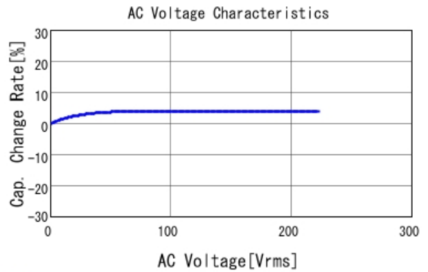
■ GRM31A7U2J100JW31 C-AC Voltage capchange, DC0V, 25.0d
