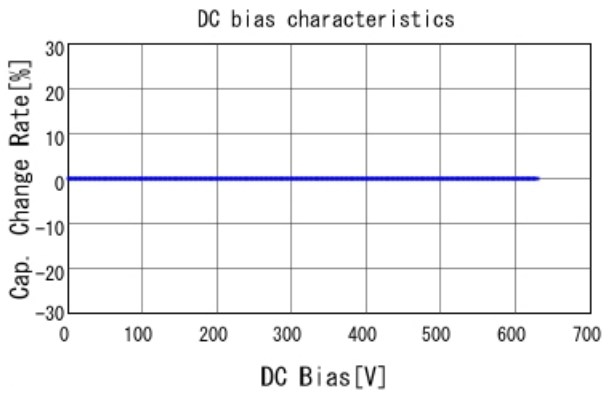
■ GRM31A7U2J100JW31 C-DC bias capchange, 25.0degC, AC1V
