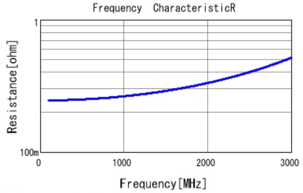
■ GRM31A7U2J100JW31 R DC0V, 25degC
