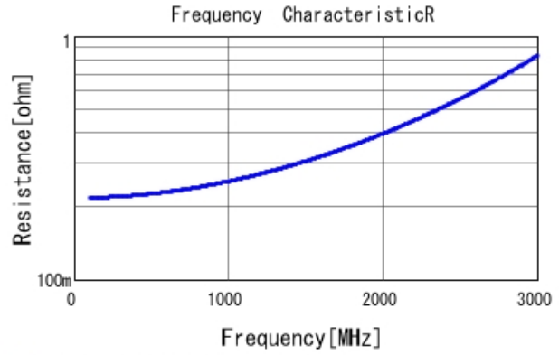
■ GRM31A7U2J120JW31 R DC0V, 25degC
