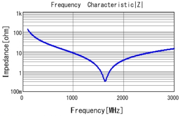
■ GRM31A7U2J120JW31 |Z| DC0V, 25degC
