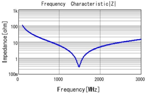
■ GRM31A7U2J150JW31 |Z| DCOV, 25degC
