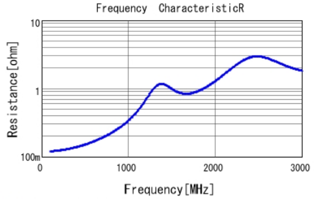
■ GRM31A7U2J151JW31 R DCOV, 25degC
