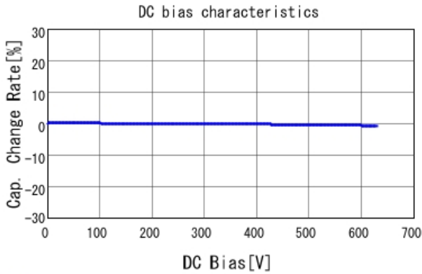
■ GRM31A7U2J151JW31 C-DC bias capchange, 25.0degC, AC1V
