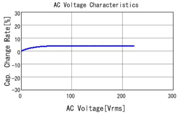
■ GRM31A7U2J151JW31 C-AC Voltage capchange, DCOV, 25.0d
