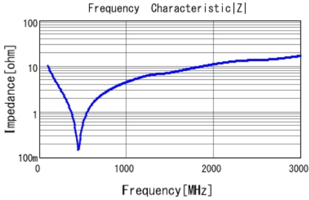
■ GRM31A7U2J151JW31 |Z| DCOV, 25degC
