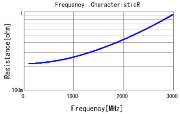
■ GRM31A7U2J220JW31 R DCOV, 25degC
