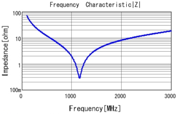
■ GRM31A7U2J220JW31 |Z| DCOV, 25degC
