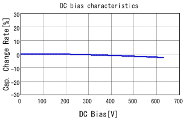
■ GRM31A7U2J391JW31 C-DC bias capchange, 25.0degC, AC1V
