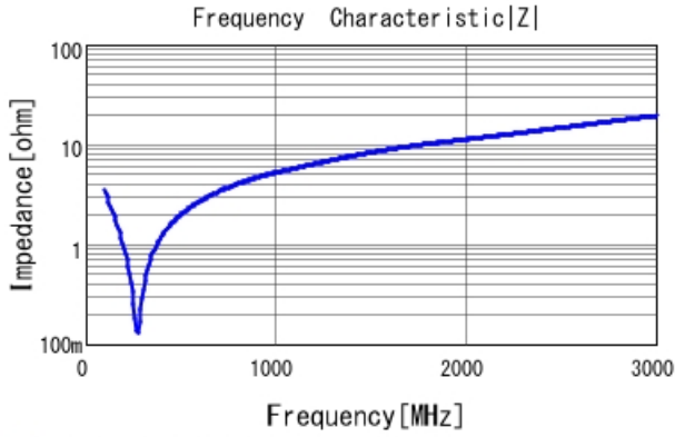
■ GRM31A7U2J391JW31 |Z| DCOV, 25degC
