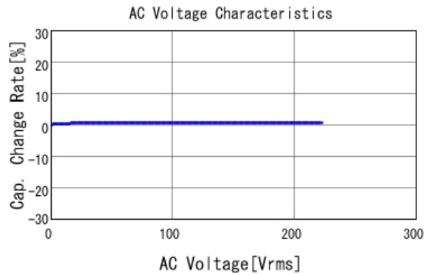
■ GRM31A7U2J391JW31 C-AC Voltage capchange, DCOV, 25.0d
