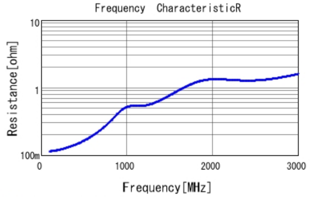
■ GRM31A7U2J391JW31 R DCOV, 25degC
