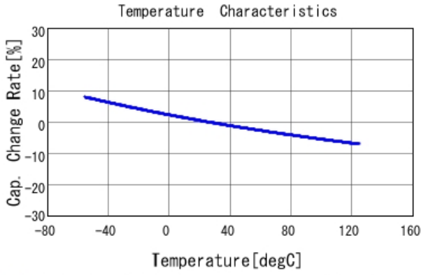
■ GRM31A7U2J561JW31 C-Temp. capchange, DCOV, AC1Vrms
