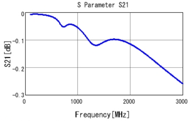
■ GRM31A7U2J561JW31 S21 DCOV, 25degC
