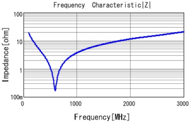
■ GRM31A7U2J820JW31 |Z| DC0V, 25degC
