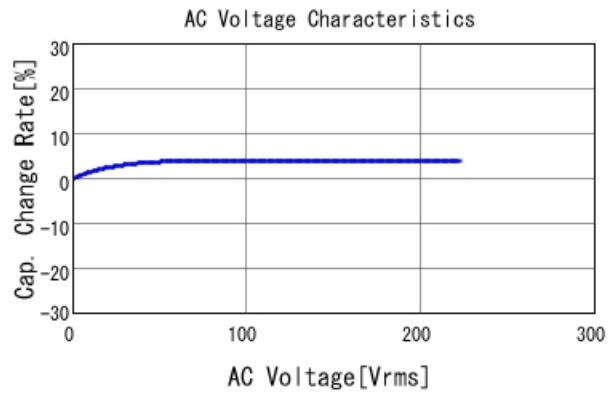
■ GRM31A7U2J820JW31 C-AC Voltage capchange, DC0V, 25.0d
