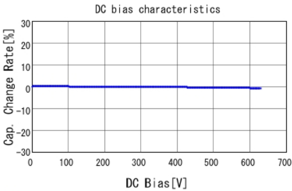
■ GRM31A7U2J820JW31 C-DC bias capchange, 25.0degC, AC1V
