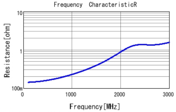
■ GRM31A7U2J820JW31 R DC0V, 25degC
