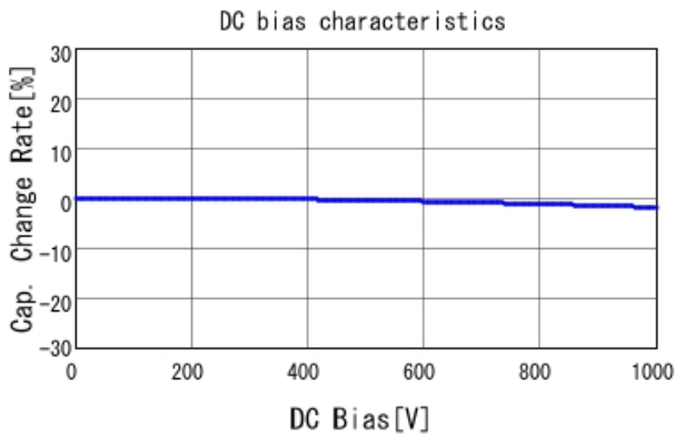
■ GRM31A7U3A121JW31 C-DC bias capchange, 25.0degC, AC1V
