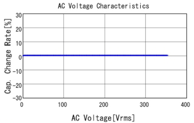
■ GRM31A7U3A121JW31 C-AC Voltage capchange, DCOV, 25.0d
