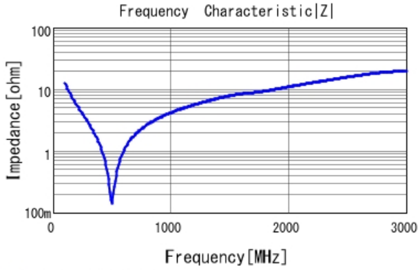
■ GRM31A7U3A121JW31 |Z| DCOV, 25degC
