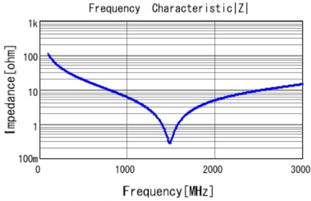
■ GRM31A7U3A150JW31 |Z| DCOV, 25degC
