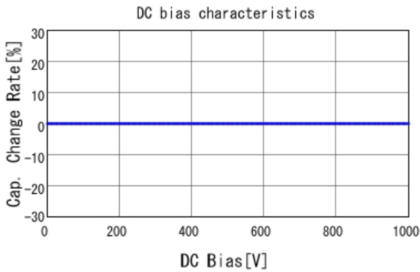
■ GRM31A7U3A150JW31 C-DC bias capchange, 25.0degC, AC1V
