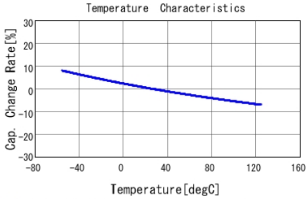
■ GRM31A7U3A150JW31 C-Temp. capchange, DCOV, AC1Vrms
