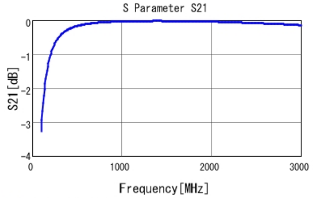
■ GRM31A7U3A150JW31 S21 DCOV, 25degC
