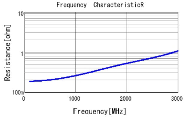
■ GRM31A7U3A270JW31 R DCOV, 25degC
