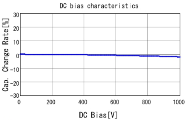
■ GRM31A7U3A270JW31 C-DC bias capchange, 25.0degC, AC1V
