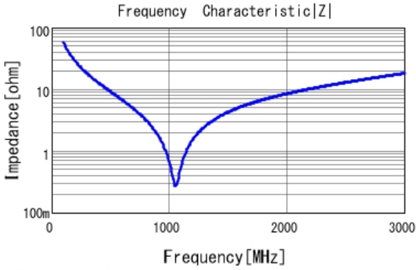
■ GRM31A7U3A270JW31 |Z| DCOV, 25degC
