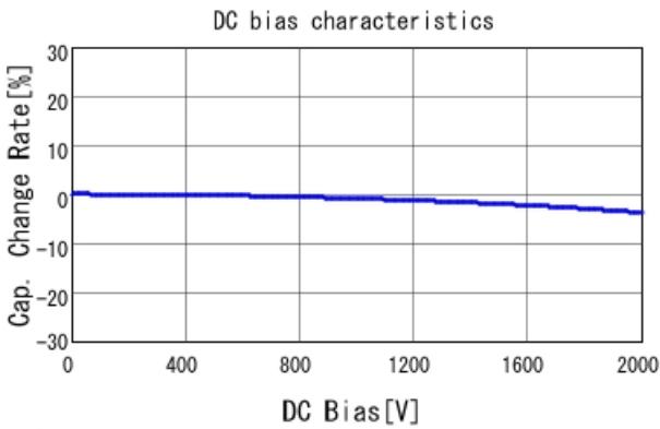
■ GRM31A7U3D270JW31 C-DC bias capchange, 25.0degC, AC1V
