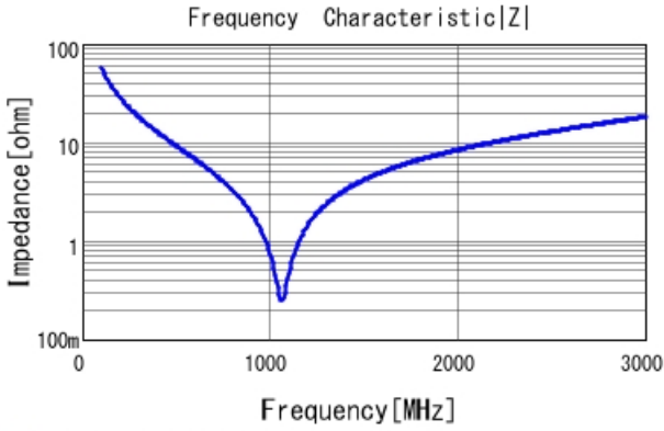
■ GRM31A7U3D270JW31 |Z| DC0V, 25degC
