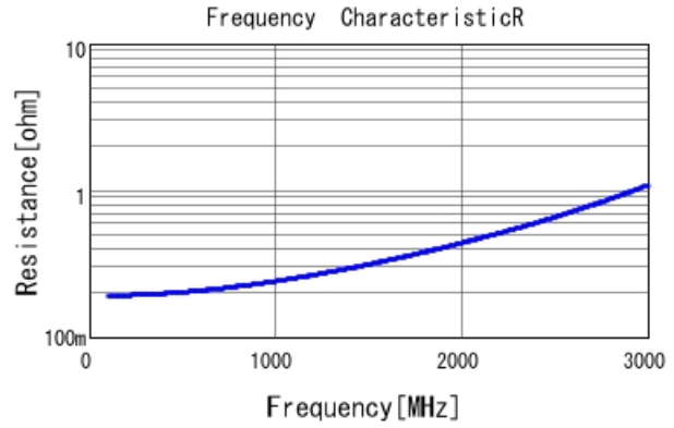
■ GRM31A7U3D270JW31 R DC0V, 25degC
