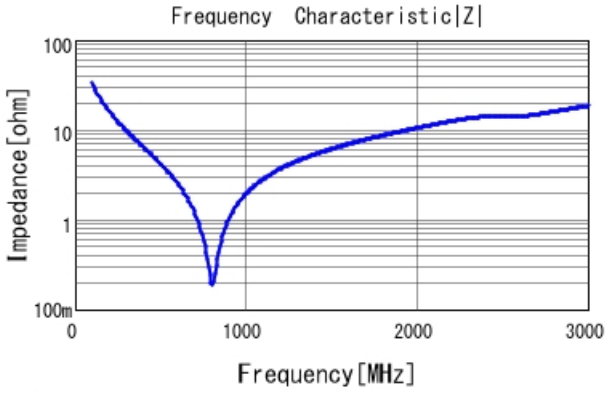
■ GRM31A7U3D470JW31 |Z| DC0V, 25degC
