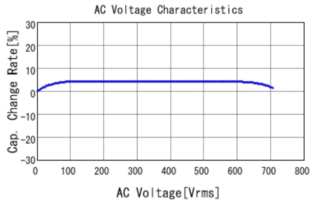
■ GRM31A7U3D470JW31 C-AC Voltage capchange, DC0V, 25.0d
