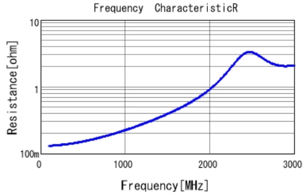
■ GRM31A7U3D470JW31 R DC0V, 25degC
