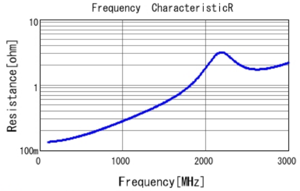
■ GRM31A7U3D560JW31 R DCOV, 25degC
