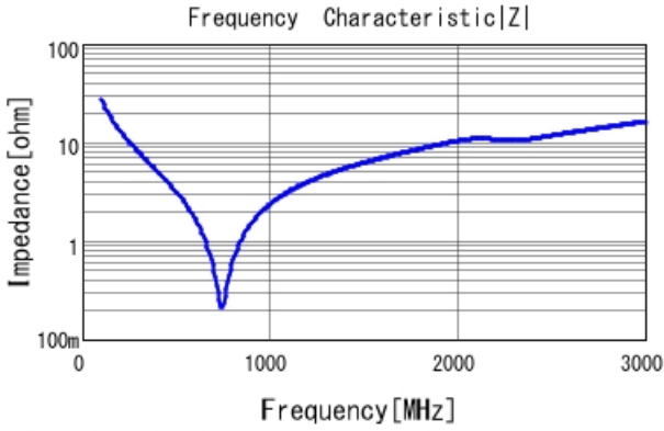
■ GRM31A7U3D560JW31 |Z| DCOV, 25degC
