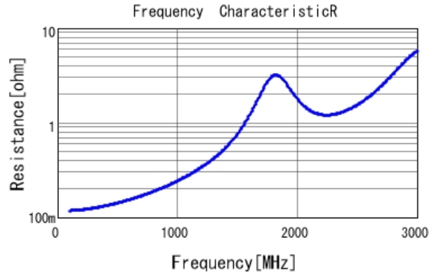
■ GRM31A7U3D680JW31 R DCOV, 25degC
