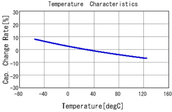
■ GRM31A7U3D680JW31 C-Temp. capchange, DCOV, AC1Vrms
