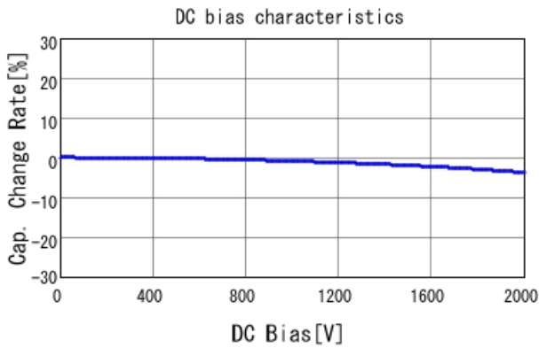
■ GRM31A7U3D680JW31 C-DC bias capchange, 25.0degC, AC1V
