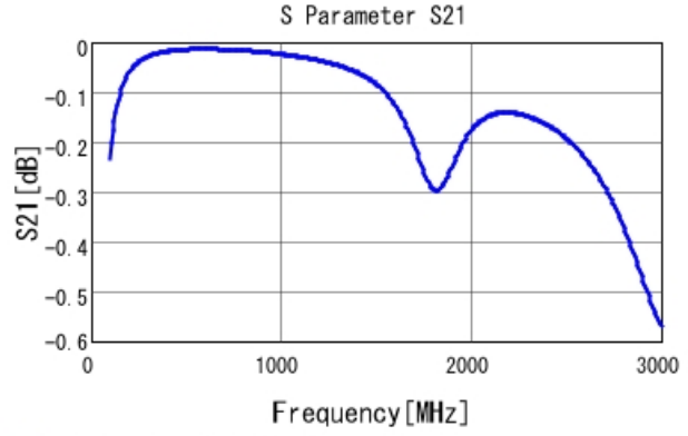
■ GRM31A7U3D680JW31 S21 DCOV, 25degC
