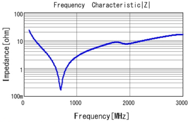
■ GRM31A7U3D680JW31 |Z| DCOV, 25degC
