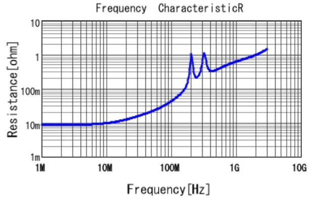
■ GRM31B7U2J332JW31 R DCOV, 25degC
