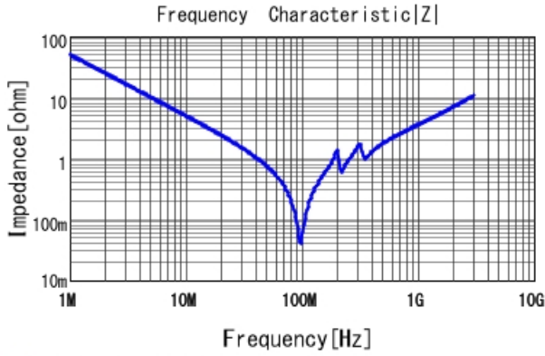
■ GRM31B7U2J332JW31 |Z| DCOV, 25degC
