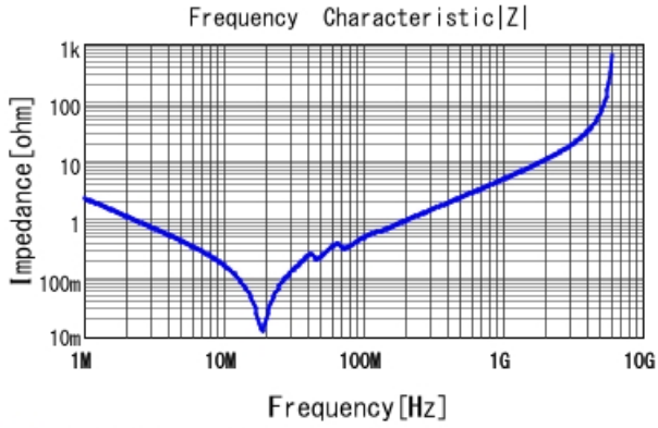
■ GRM31C5C2A683JA01 |Z| DCOV, 25degC
