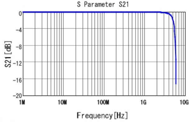
■ GRM31C5C2A683JA01 S21 DCOV, 25degC
