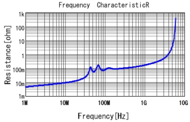
■ GRM31C5C2A683JA01 R DCOV, 25degC
