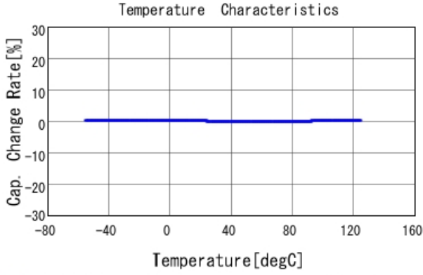
■ GRM31C5C2A683JA01 C-Temp. capchange, DCOV, AC1Vrms
