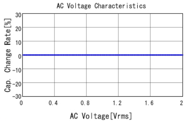
■ GRM31C5C2A683JA01 C-AC Voltage capchange, DCOV, 25.0d
