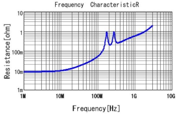
■ GRM31C7U2J392JW32 R DCOV, 25degC
