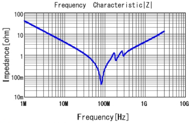
■ GRM31C7U2J392JW32 |Z| DCOV, 25degC
