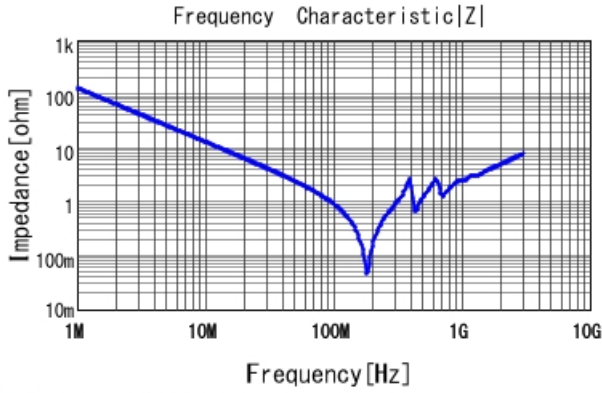
■ GRM32B7U3A122JW31 |Z| DCOV, 25degC
