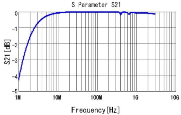
■ GRM32B7U3A122JW31 S21 DCOV, 25degC
