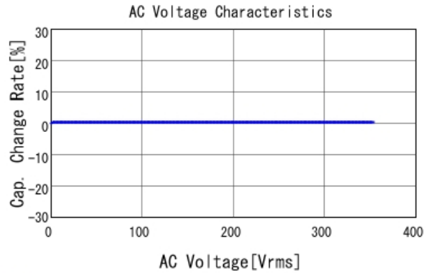
■ GRM32B7U3A122JW31 C-AC Voltage capchange, DCOV, 25.0d
