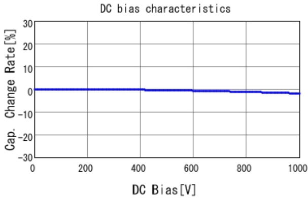
■ GRM32B7U3A122JW31 C-DC bias capchange, 25.0degC, AC1V
