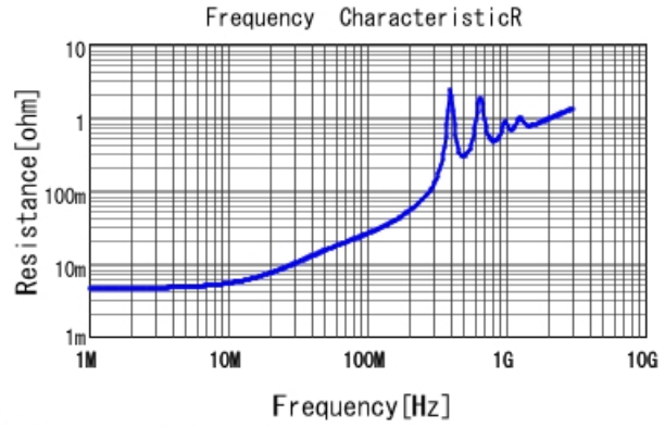
■ GRM32B7U3A122JW31 R DCOV, 25degC
