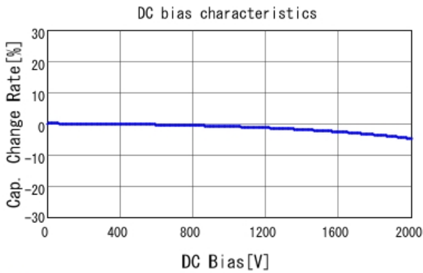
■ GRM32B7U3D181JW31 C-DC bias capchange, 25.0degC, AC1V
