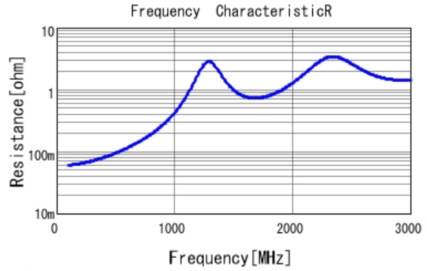
■ GRM32B7U3D181JW31 R DCOV, 25degC
