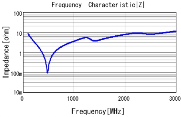
■ GRM32B7U3D181JW31 |Z| DCOV, 25degC
