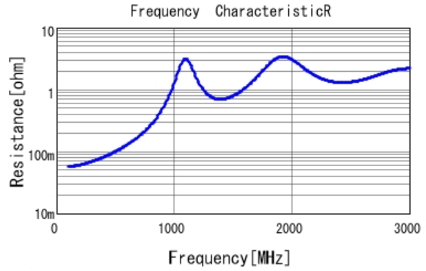
■ GRM32B7U3D221JW31 R DC0V, 25degC
