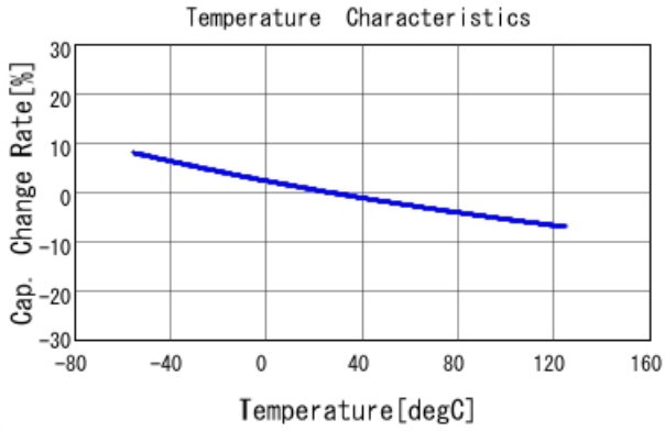
■ GRM32B7U3D221JW31 C-Temp. capchange, DCOV, AC1Vrms
