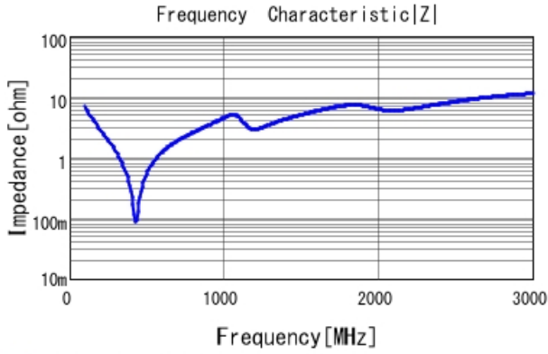
■ GRM32B7U3D221JW31 |Z| DC0V, 25degC
