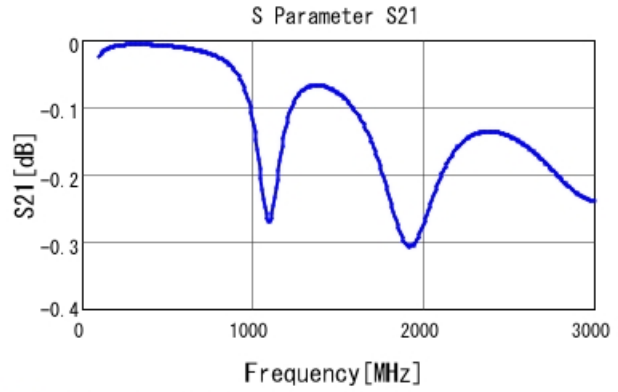
■ GRM32B7U3D221JW31 S21 DCOV, 25degC
