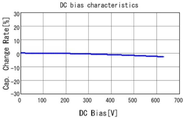
■ GRM32D7U2J103JW31 C-DC bias capchange, 25.0degC, AC1V
