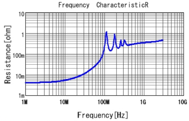
■ GRM32D7U2J103JW31 R DCOV, 25degC
