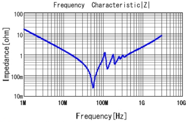
■ GRM32D7U2J103JW31 |Z| DCOV, 25degC
