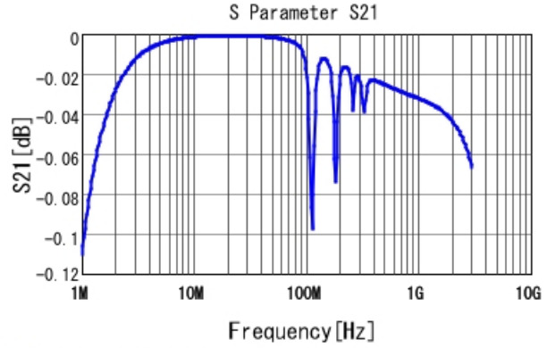
■ GRM32D7U2J103JW31 S21 DCOV, 25degC
