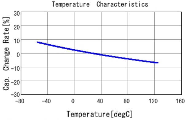
■ GRM32D7U2J103JW31 C-Temp. capchange, DCOV, AC1Vrms
