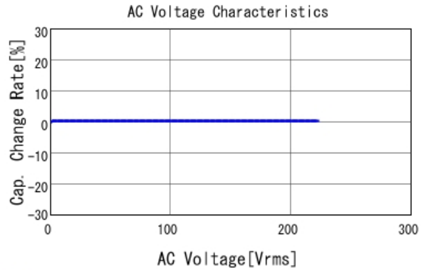
■ GRM32D7U2J103JW31 C-AC Voltage capchange, DCOV, 25.0d
