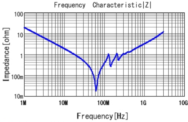
■ GRM32D7U2J822JW31 |Z| DCOV, 25degC
