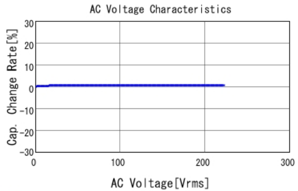
■ GRM32D7U2J822JW31 C-AC Voltage capchange, DCOV, 25.0d
