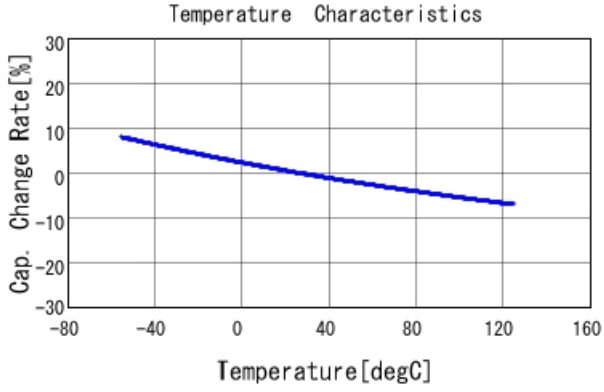
■ GRM32D7U2J822JW31 C-Temp. capchange, DCOV, AC1Vrms
