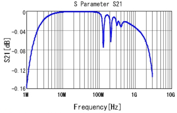
■ GRM32D7U2J822JW31 S21 DCOV, 25degC
