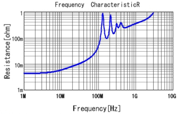
■ GRM32D7U2J822JW31 R DCOV, 25degC
