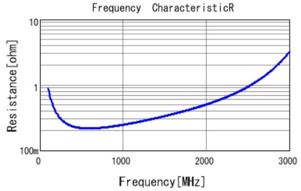
■ GRM42A7U3F220JW31 R DC0V, 25degC
