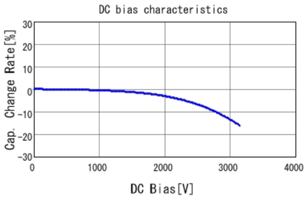
■ GRM42A7U3F220JW31 C-DC bias capchange, 25.0degC, AC1V
