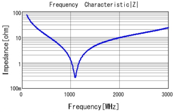
■ GRM42A7U3F220JW31 |Z| DC0V, 25degC
