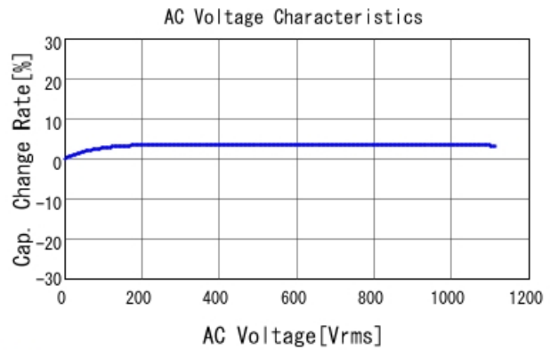
■ GRM42A7U3F220JW31 C-AC Voltage capchange, DC0V, 25.0d
