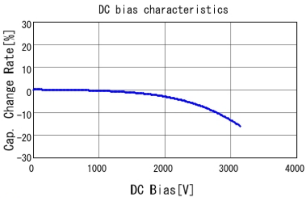
■ GRM42A7U3F470JW31 C-DC bias capchange, 25.0degC, AC1V
