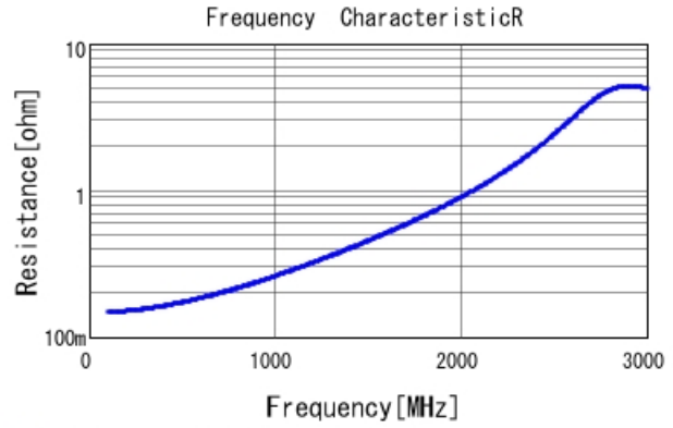
■ GRM42A7U3F470JW31 R DCOV, 25degC
