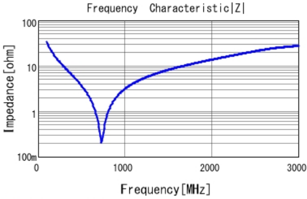
■ GRM42A7U3F470JW31 |Z| DCOV, 25degC
