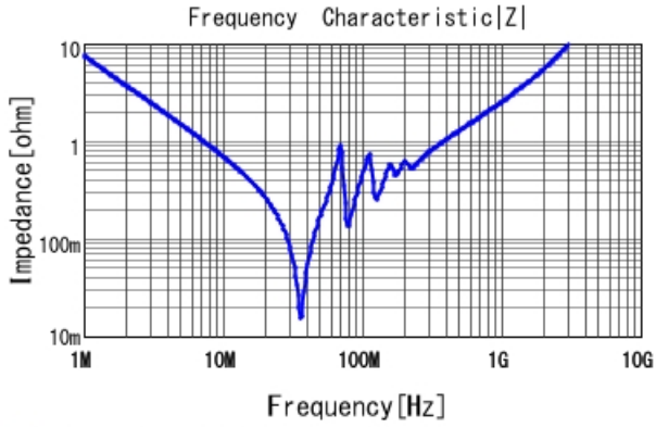
■ GRM43D7U2J223JW31 |Z| DCOV, 25degC
