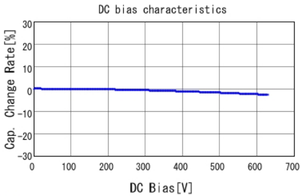
■ GRM43D7U2J223JW31 C-DC bias capchange, 25.0degC, AC1V
