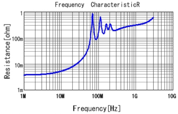
■ GRM43D7U2J223JW31 R DCOV, 25degC
