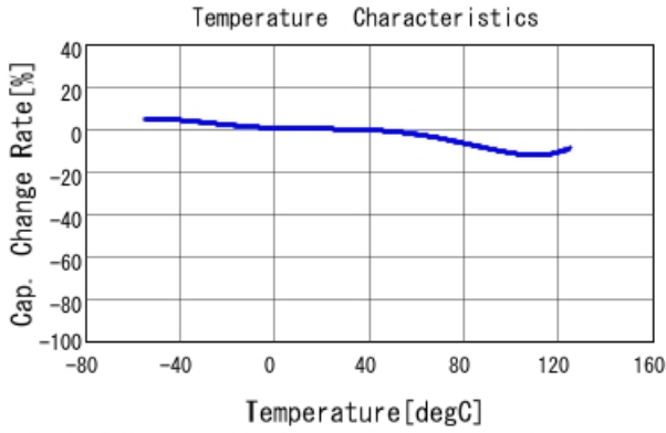
■ GRM43QR72E154KW01 C-Temp. capchange, DCOV, AC1Vrms
