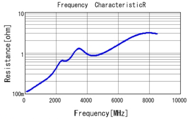
■ GRT0335C1E101FA02 R DC0V, 25degC
