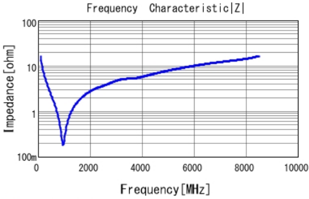
■ GRT0335C1E101FA02 |Z| DC0V, 25degC
