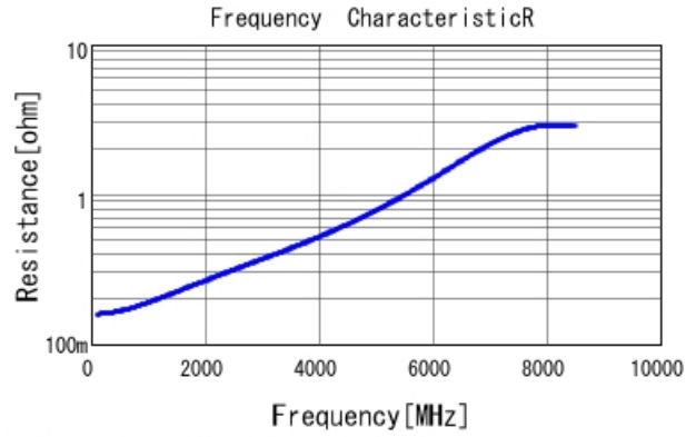
■ GRT0335C1E180FA02 R DC0V, 25degC
