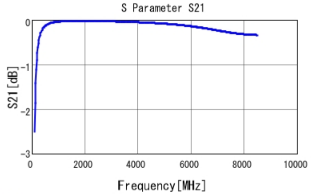
■ GRT0335C1E180FA02 S21 DCOV, 25degC
