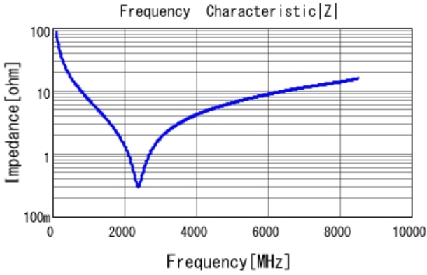
■ GRT0335C1E180FA02 |Z| DC0V, 25degC
