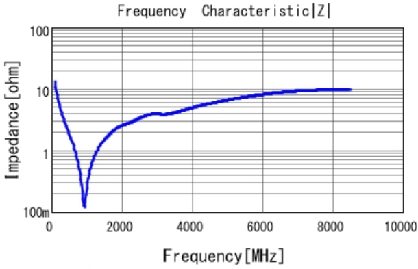
■ GRT0335C1H121FA02 |Z| DC0V, 25degC
