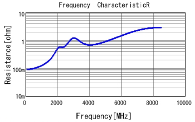
■ GRT0335C1H121FA02 R DC0V, 25degC
