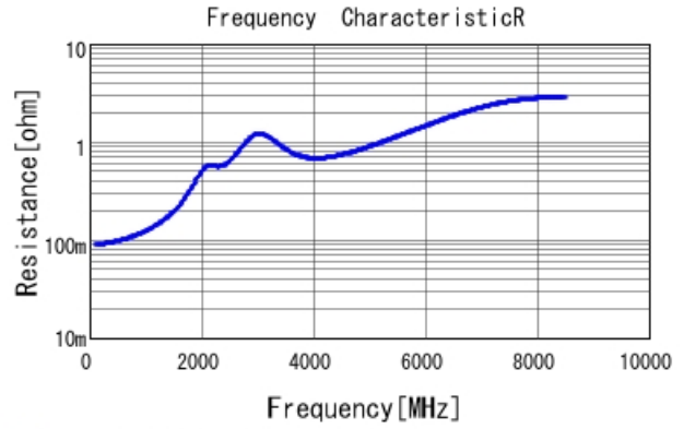
■ GRT0335C1H121JA02 R DC0V, 25degC
