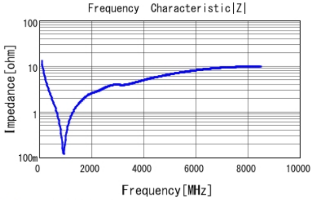
■ GRT0335C1H121JA02 |Z| DC0V, 25degC
