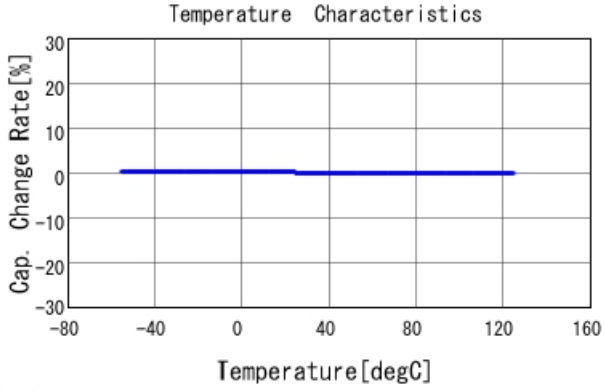
■ GRT0335C1H1R0CA02 C-Temp. capchange, DCOV, AC1Vrms
