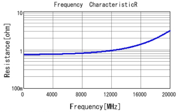
■ GRT0335C1H1R0CA02 R DCOV, 25degC
