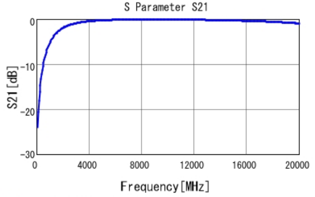
■ GRT0335C1H1R0CA02 S21 DCOV, 25degC
