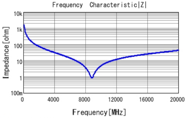
■ GRT0335C1H1R0CA02 |Z| DCOV, 25degC
