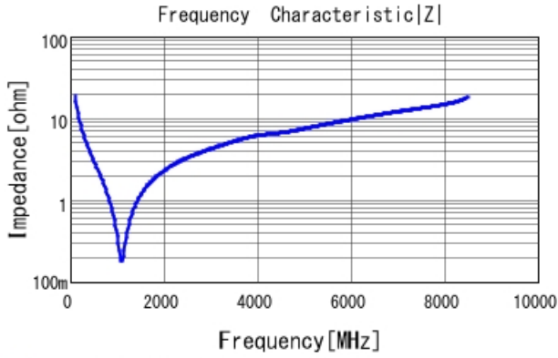
■ GRT0335C1H820FA02 |Z| DC0V, 25degC
