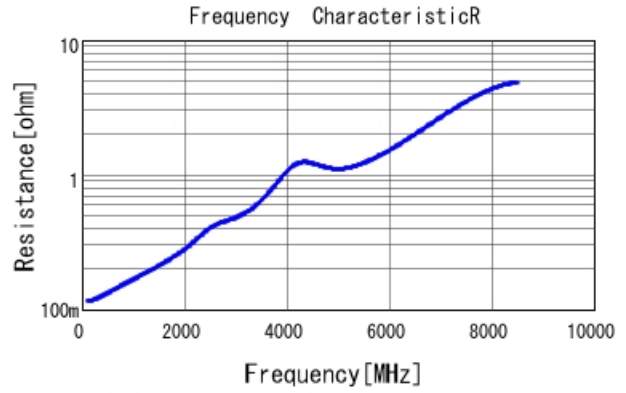
■ GRT0335C1H820FA02 R DC0V, 25degC
