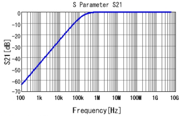
■ GRT033R71A103KE01 S21 DCOV, 25degC
