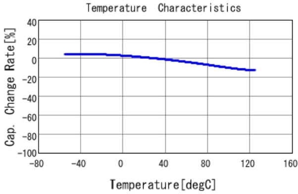
■ GRT033R71A103KE01 C-Temp. capchange, DCO. 0V, AC1. 0Vrm
