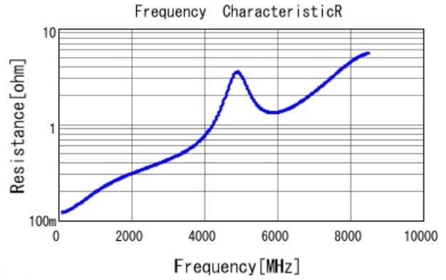
■ GRT1555C1E120JA02 R DC0V, 25degC
