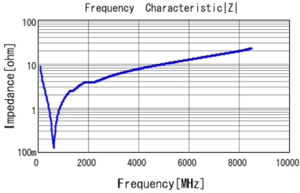
■ GRT1555C1H181JA02 |Z| DCOV, 25degC
