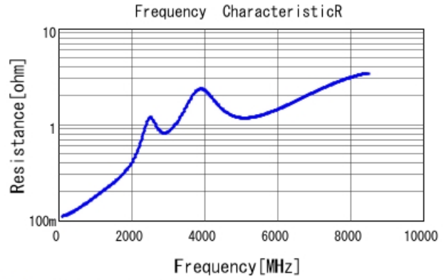
■ GRT1555C1H560JA02 R DC0V, 25degC
