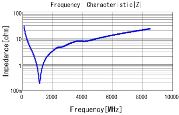
■ GRT1555C1H560JA02 |Z| DC0V, 25degC
