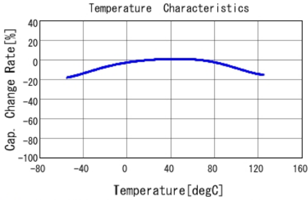
■ GRT155C71A105KE13 C-Temp. capchange, DCO. 0V, ACO. 2Vrm
