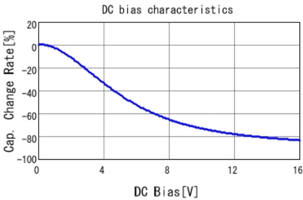
■ GRT155C81C105KE13 C-DC bias capchange, 25.0degC, AC1V
