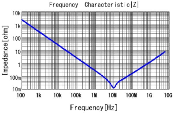
■ GRT155C81C105KE13 |Z| DC0V, 25degC
