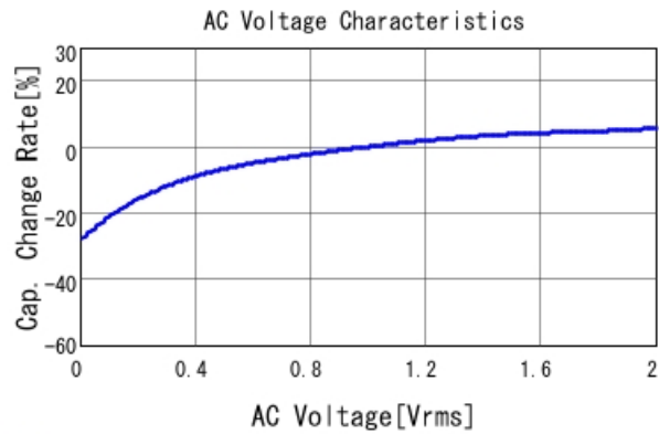
■ GRT155C81C105KE13 C-AC Voltage capchange, DC0V, 25.0d
