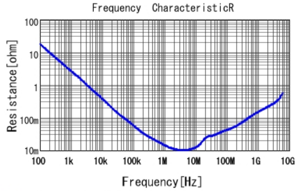
■ GRT155C81C105KE13 R DC0V, 25degC
