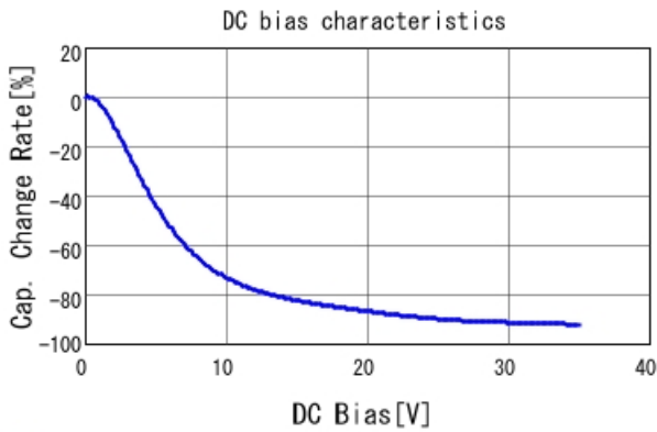
■ GRT155R6YA105KE13 C-DC bias capchange, 25.0degC, AC1V
