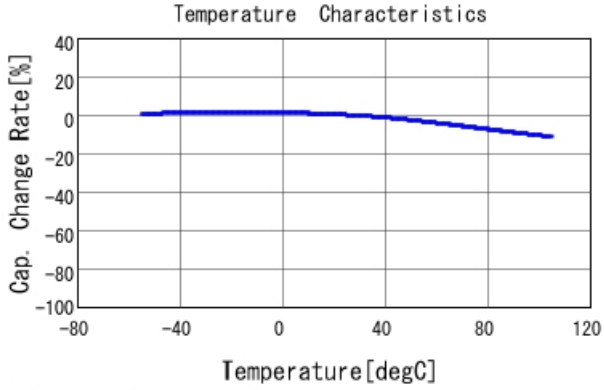
■ GRT32DC81H335KE01 C-Temp. capchange, DCO. 0V, AC1. 0Vrm
