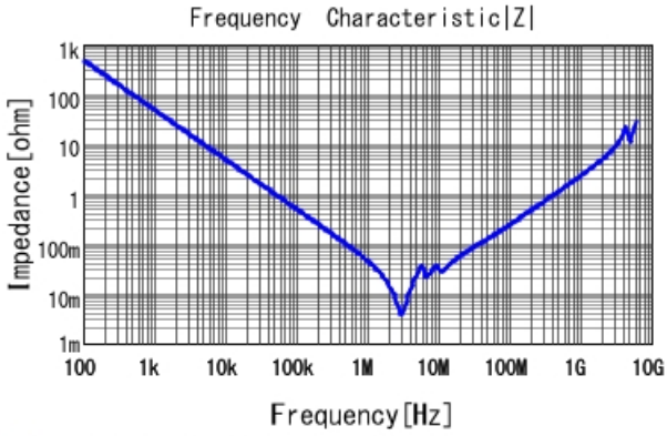
■ GRT32DR61H335KE01 |Z| DC0V, 25degC
