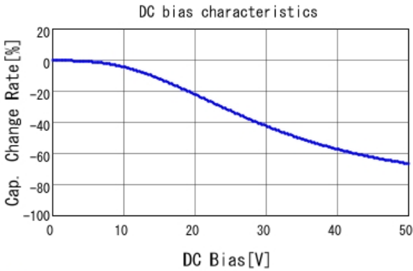
■ GRT32DR61H335KE01 C-DC bias capchange, 25.0degC, AC1.
