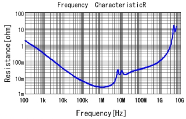
■ GRT32DR61H335KE01 R DC0V, 25degC
