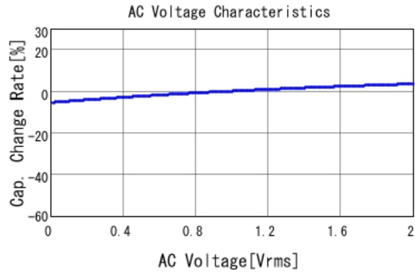
■ GRT32DR61H335KE01 C-AC Voltage capchange, DC0V, 25.0d
