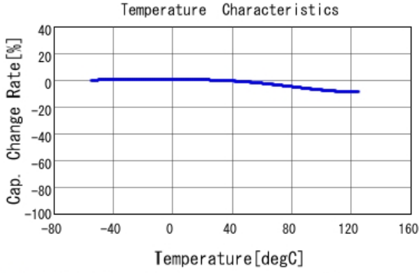
■ KRM55QR71J106KH01 C-Temp. capchange, DCOV, AC1Vrms
