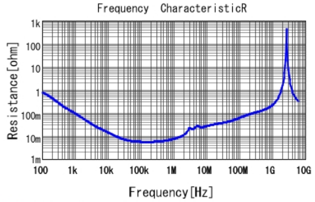
■ KRM55QR71J106KH01 R DCOV, 25degC
