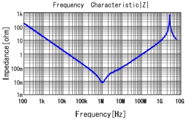
■ KRM55QR71J106KH01 |Z| DCOV, 25degC
