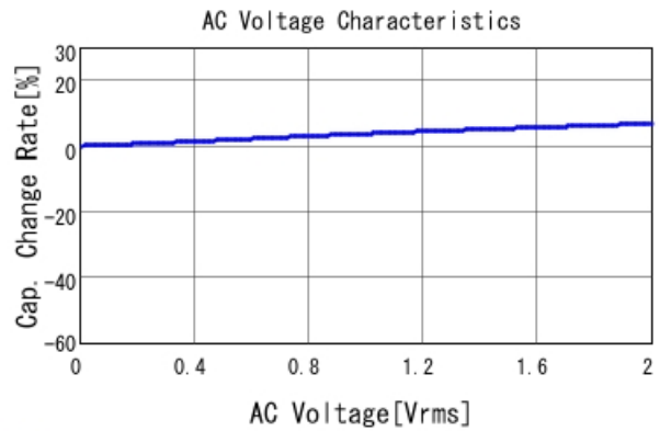
■ KRM55QR71J106KH01 C-AC Voltage capchange, DCOV, 25.0d
