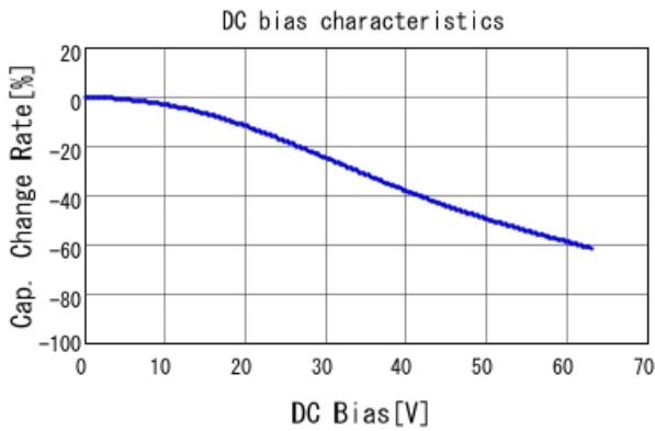
■ KRM55QR71J106KH01 C-DC bias capchange, 25.0degC, AC1V
