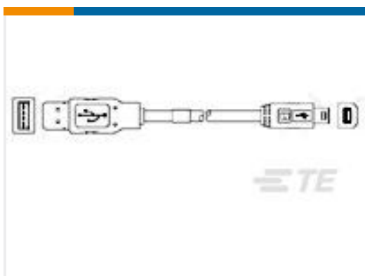
TE Part #1487597-2 USB, A-B, 25/22, BLACK, 2.5M
