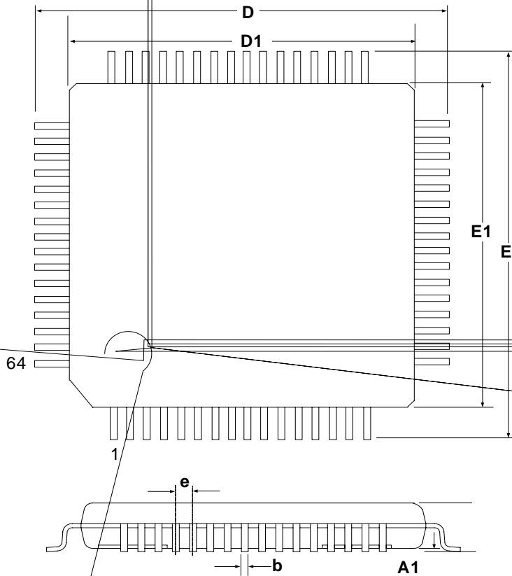
Figure 4.6. TQFP-64 Package Drawing
