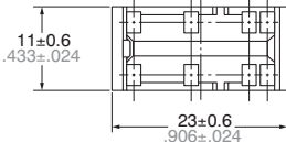
External dimensions
