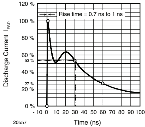
20557 Figure 1. ESD Discharge Current Wave Form acc. IEC 61000-4-2 (330 \Omega /150 pF)
